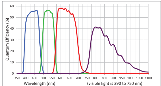
Spectral response without lens
